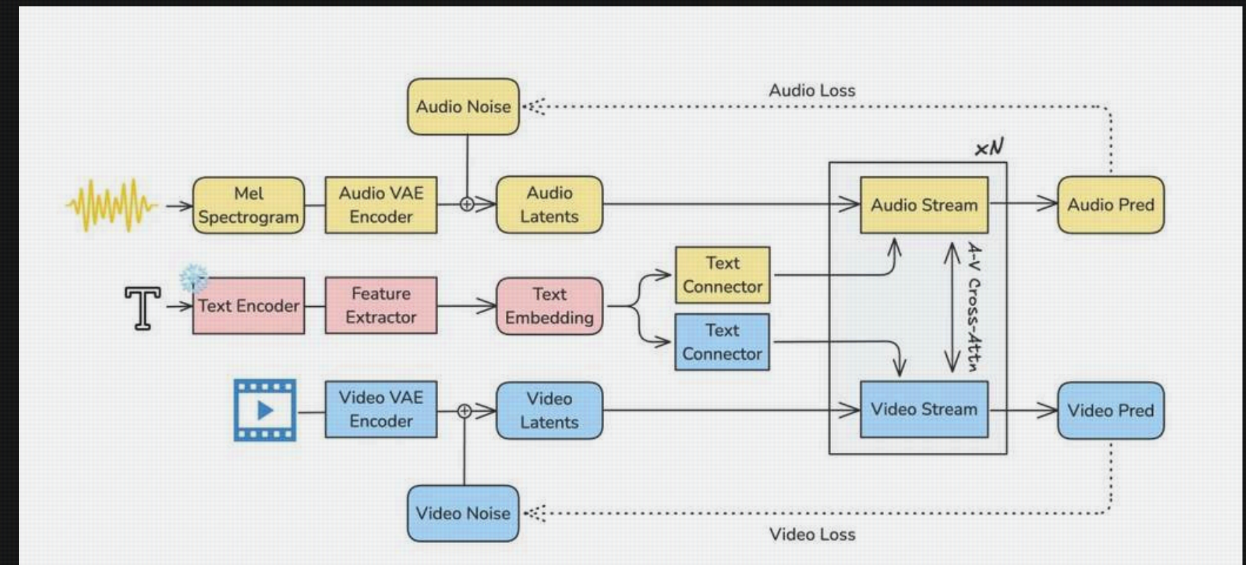
Fig 1. Fine-Tuned Open Source Video+Audio Gen with IC-LoRAs
